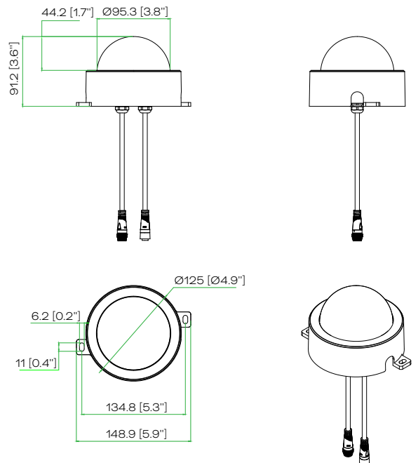
Bottom cable feed (customized)
