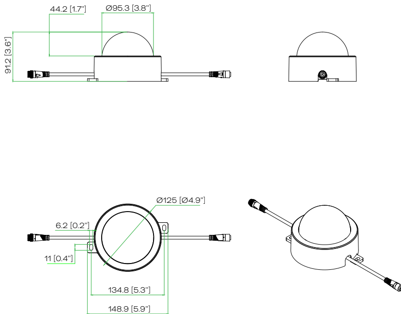
Side cable feed (standard)
