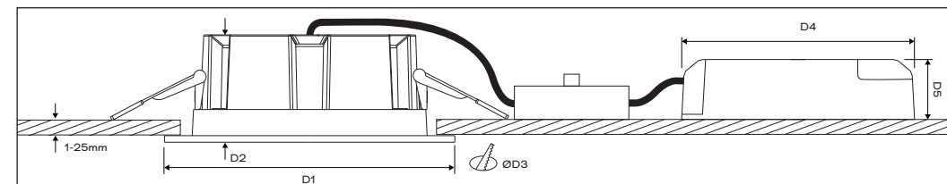
Product Dimensions
